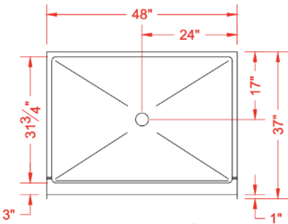
TOP VIEW - SCALE \frac{3}{8} " = 1'-0"
